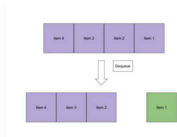
Figura 2. dequeue
